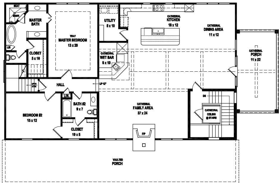
SECOND LEVEL FLOOR PLAN
