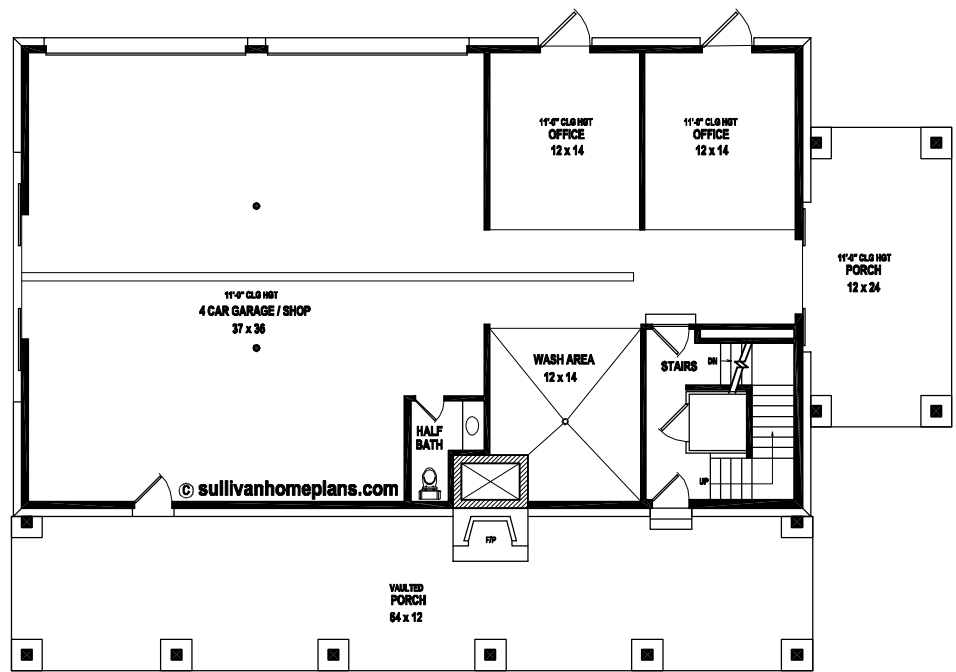
FIRST LEVEL FLOOR PLAN
